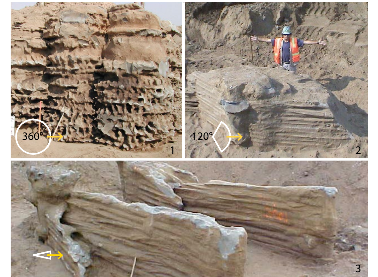
1. Secant columns. | 2. Partial column 120°. | 3. Mono-direction panel.
